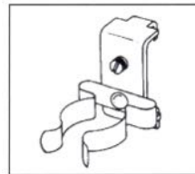
Fjäderklämma K4001 Ø 13 mm K4002 Ø 16 mm K4003 Ø 19 mm K4004 Ø 25 mm K4005 Ø 28 mm K4006 Ø 32 mm K4007 Ø 38 mm
